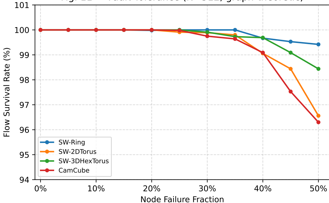
Fig. 11 — Fault Tolerance (N=512, graph-theoretic)
